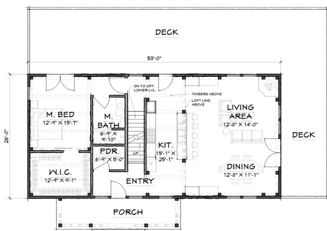
FIRST FLOOR - 1,378 SQ.FT.
