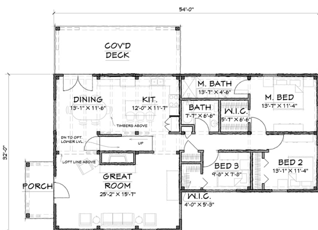
FIRST FLOOR - 1471 SQ.FT.
