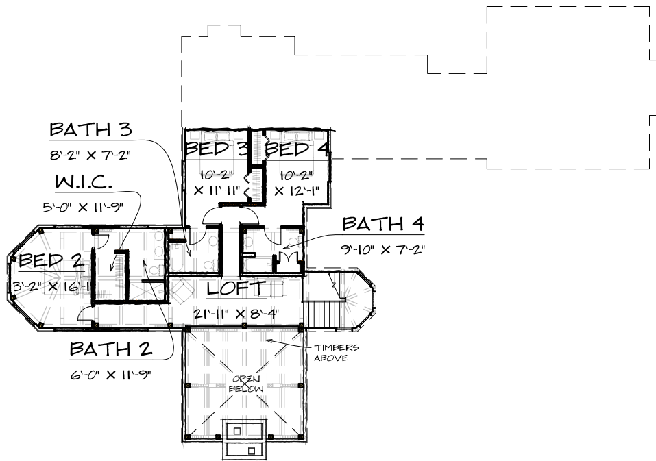
SECOND FLOOR - 1157 SQ. FT.
