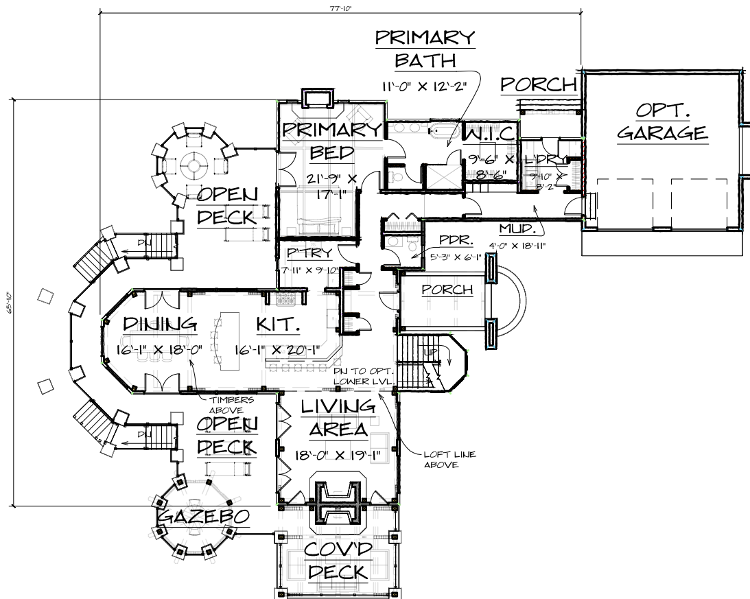
FIRST FLOOR - 2359 SQ. FT.
