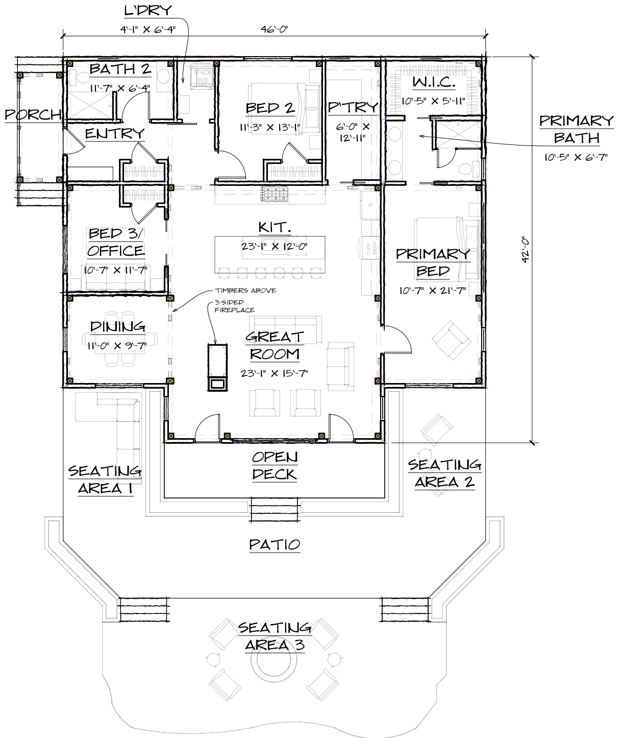
FIRST FLOOR - 1800 SQ. FT.
