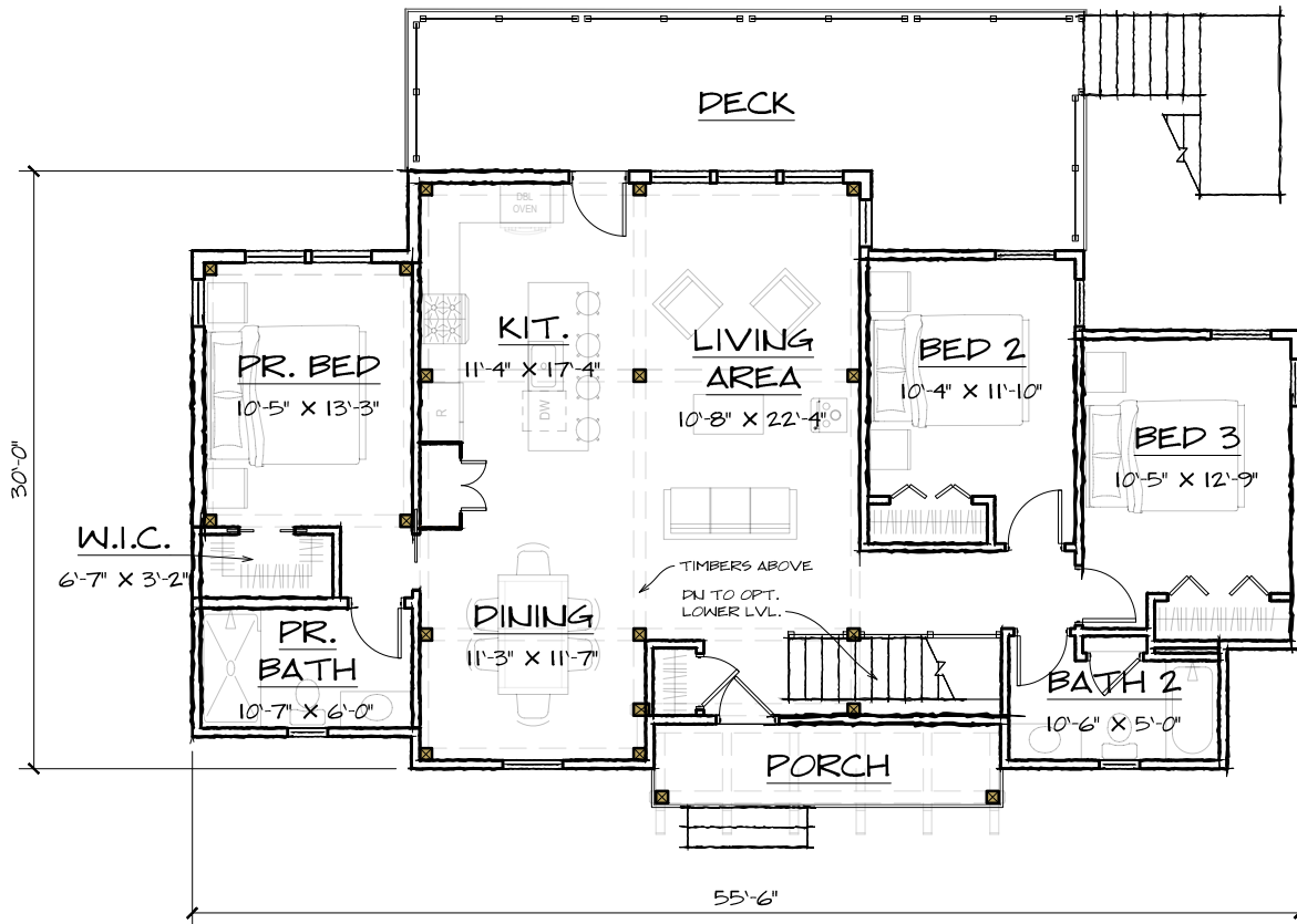
FIRST FLOOR - 1405 SQ. FT.
