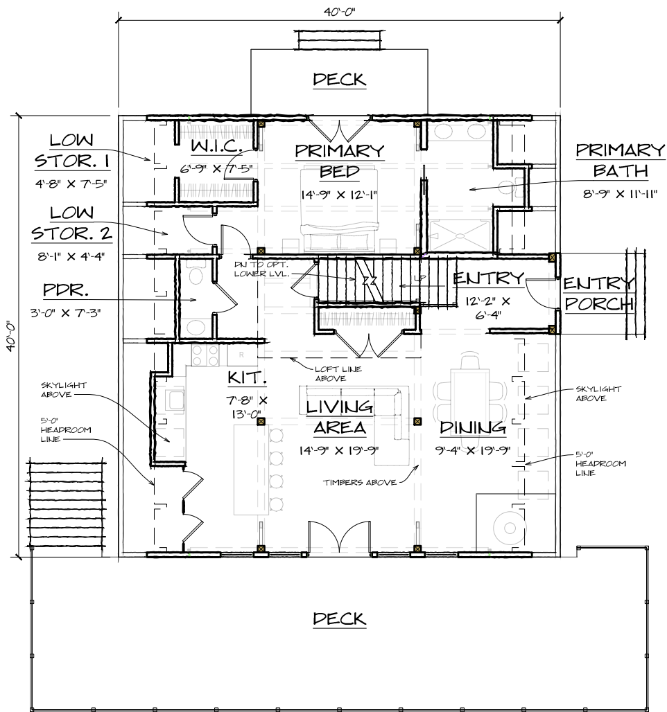
FIRST FLOOR - 1323 SQ. FT.
