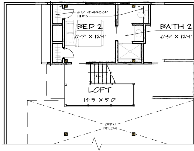
SECOND FLOOR - 361 SQ. FT.
