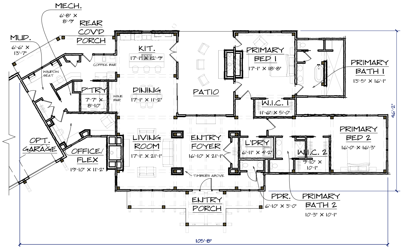
FIRST FLOOR - 3226 SQ. FT.
